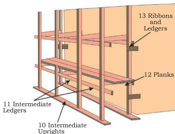
Fig. 3.6: Double Scaffolding
