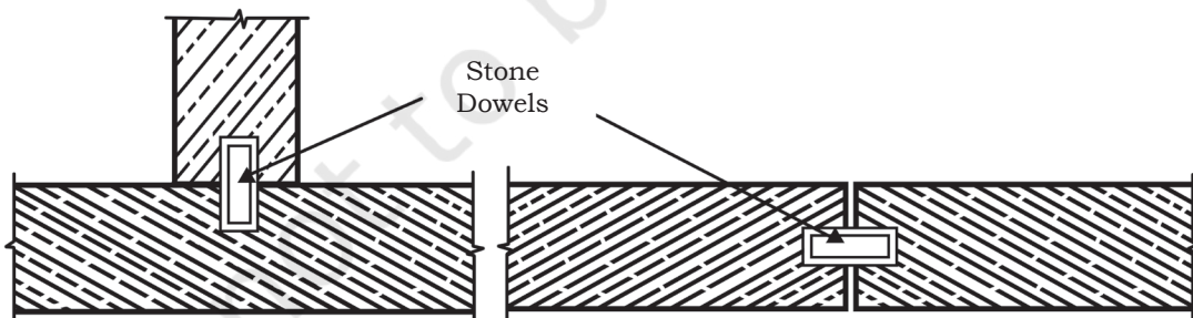
Fig. 1.24: Dowelled joint
