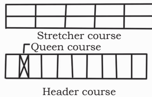
Fig. 2.11: English bond
