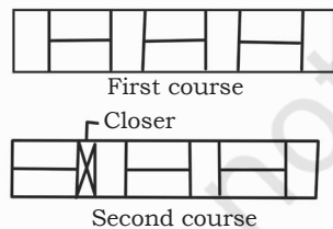
Fig. 2.12: Flemish bond
