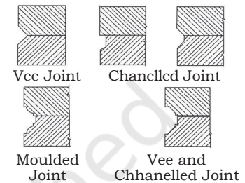
Fig. 1.22: Rusticated joint
