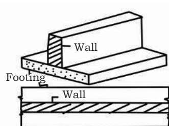
Fig. 2.14: Simple footing in brick work
