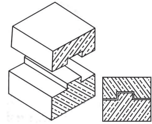
Fig. 1.21: Tabled joint
